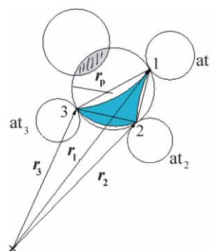
Figure 1. The probe atom with radius r_p sits between the three molecule atoms at_1 , at_2 , at_3 . If there are no steric clashes (overlaps) of the probe with nearby atoms, then a triangle is drawn between the vectors r_1 , r_2 , r_3 , ( i.e. , between the points of tangency numbered 1, 2 and 3). Its projection onto the curved probe atom surface, which forms a concave patch, is colored blue. If a steric overlap (colored grey) of the probe with a nearby atom exists, then this position of the probe is rejected.
